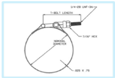
Military, Grade T Clamp
